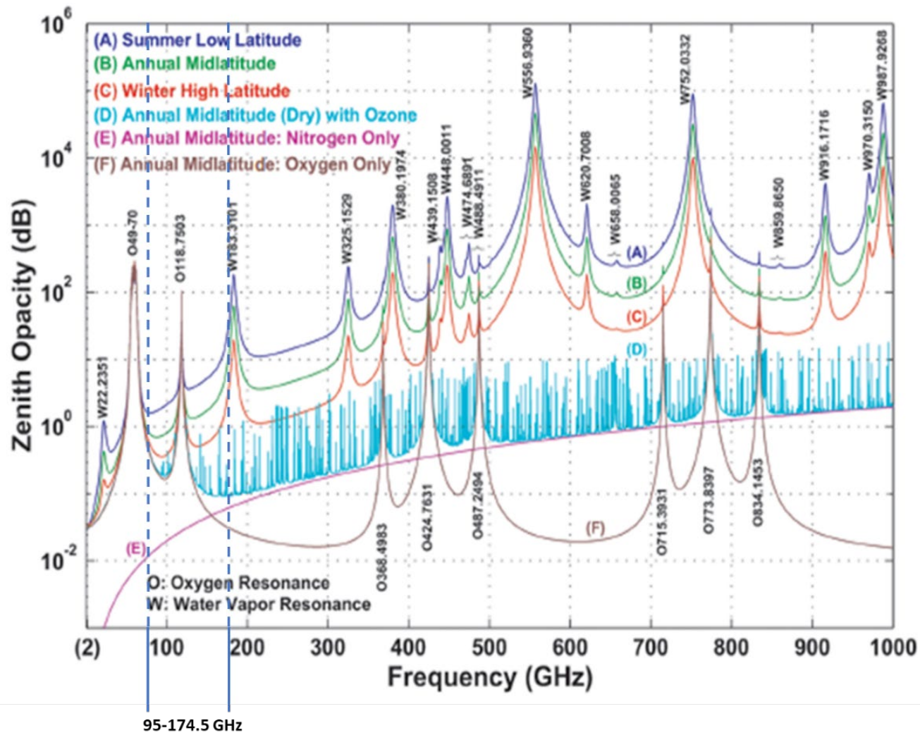
Figure 7 Atmospheric Absorption Effects (The zenith opacity is the vertically integrated absorption coefficient [Recommendation ITU-R P.676-13 (08/2022) Attenuation by atmospheric gases and related effects])
