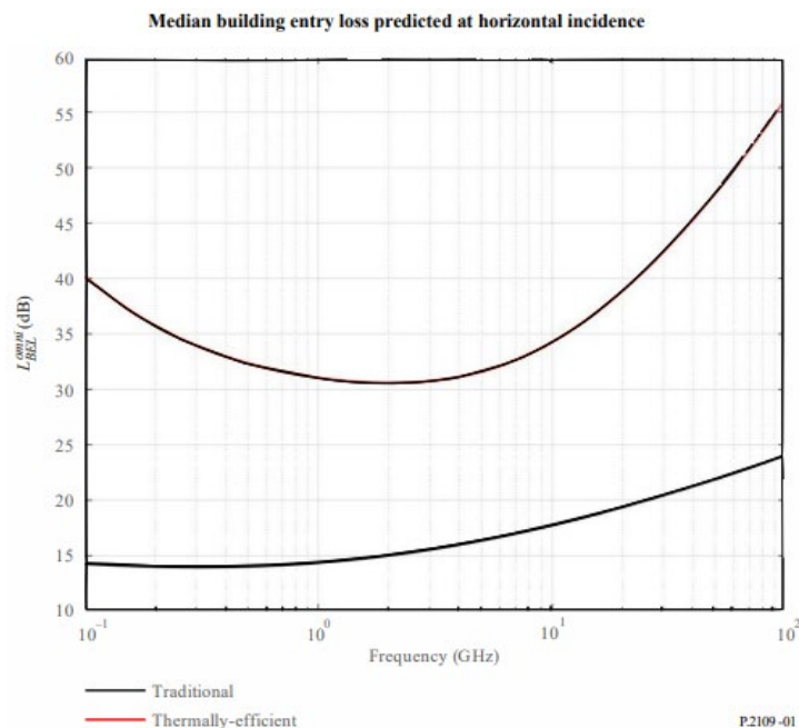
Figure 6 Median Building Entry Loss
